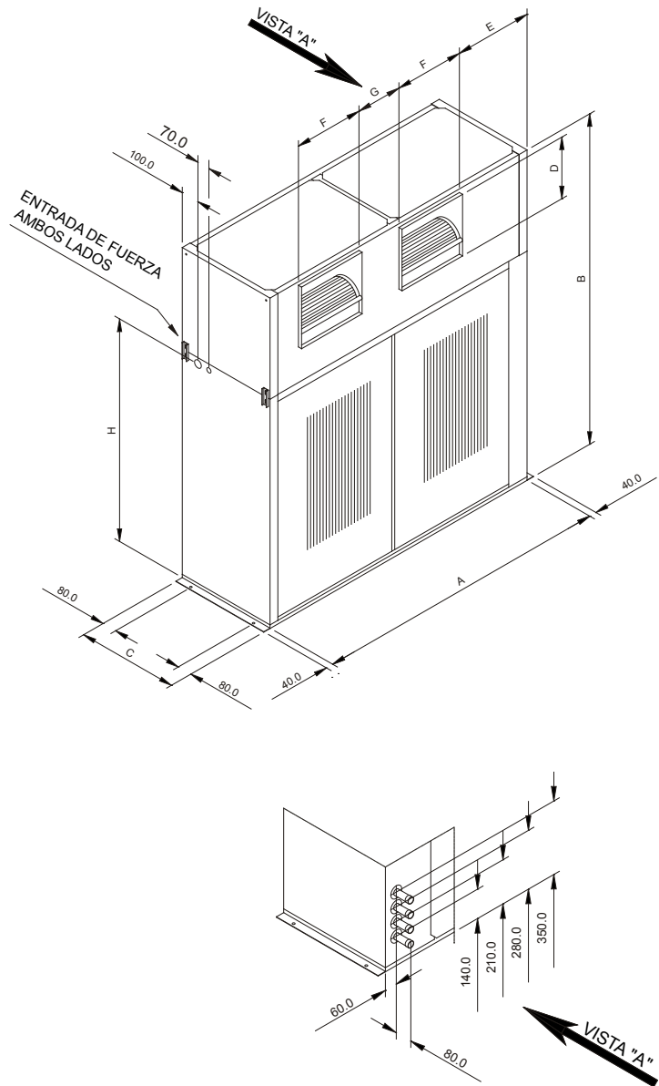
Fig. XI 38 - Dimensional TRCE
